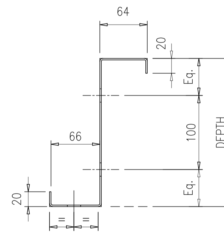
SECTION X-X
