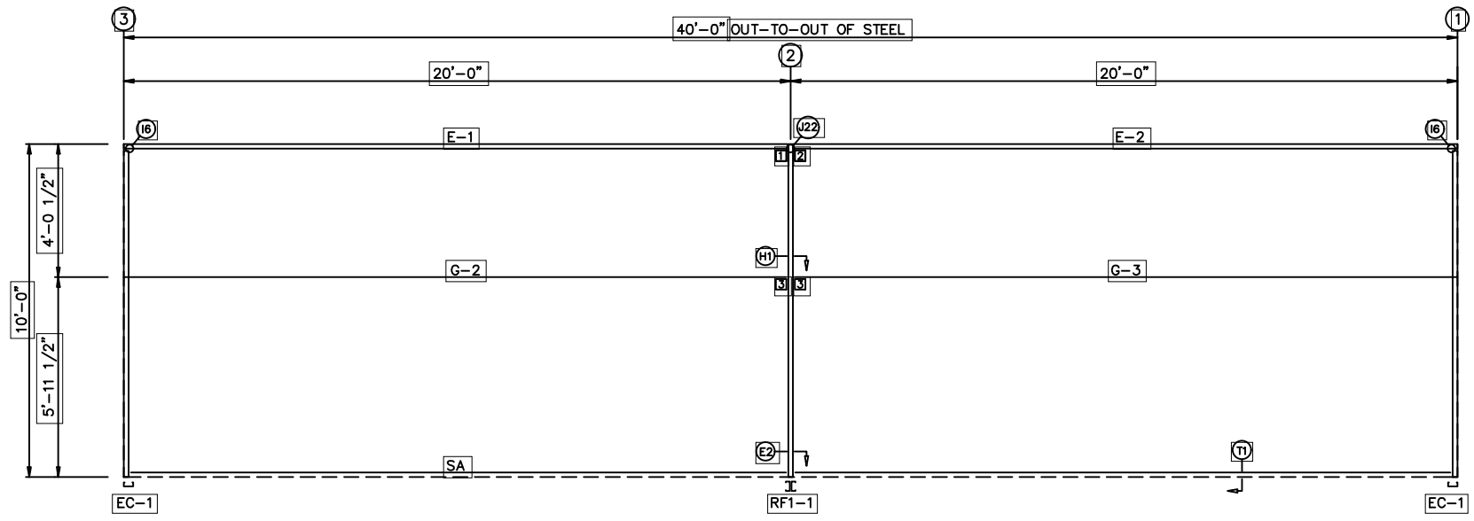
SIDEWALL FRAMING: FRAME LINE D
