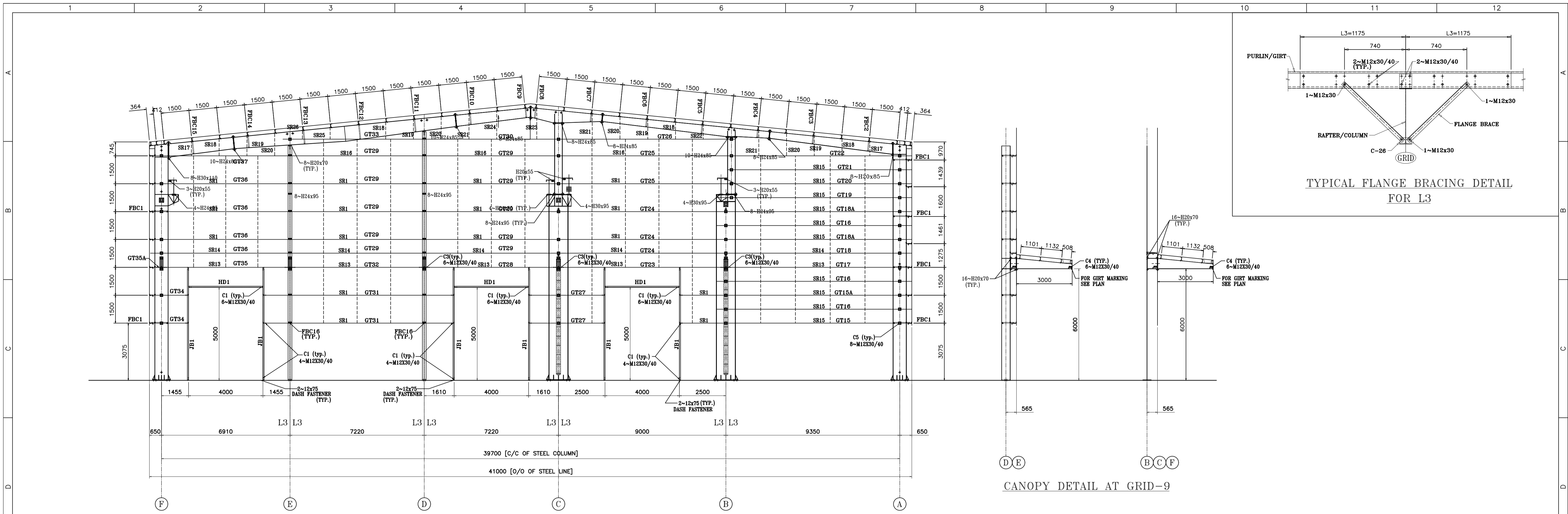
END WALL ELEVATION ALONG GRID-9
